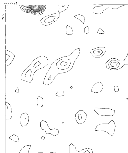
Figure 4 Native Patterson calculated using all X-ray data from crystal form Bsp~P-II. The section shown is of w = 0.5 and is plotted across the asymmetric unit for space group P2_12_12_1 . The peak at u = 0.12 , v = 0 , w = 0.5 is some 11% of the origin height and strongly suggests that there are two molecules in the asymmetric unit that are in approximately the same orientation.
