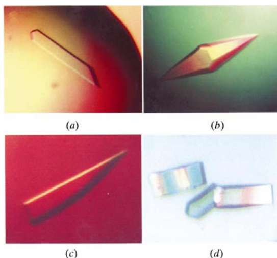
Figure 2 Crystal photomicrographs. (a) Bst SpoIIAA-II, (b) Bst SpoIIAA~P, (c) Bsp SpoIIAA and (d) Bsp SpoIIAA~P-II.
